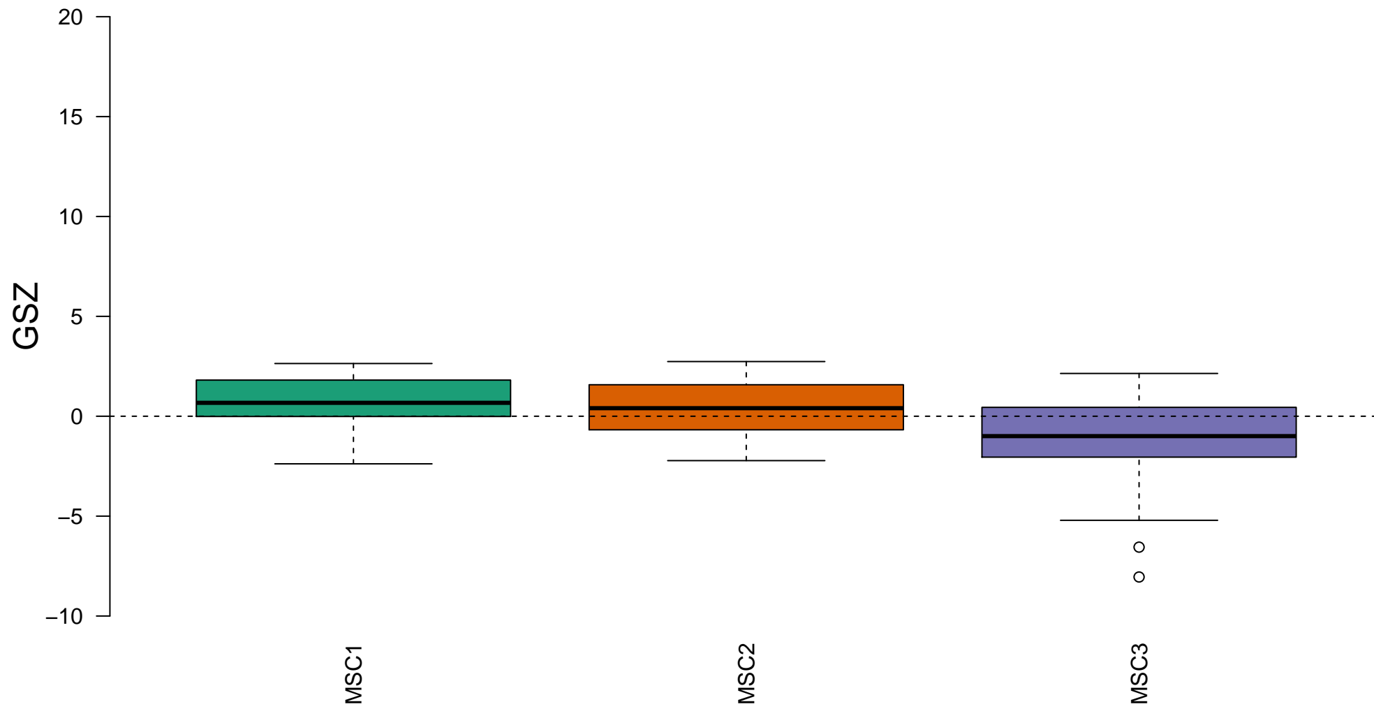
CARO_OxPhos_vs_BCR_UP
